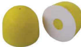
UH301 UH302 3" Water Feed Pad Center Hole: 7/8" Backing: Vinyl or Velcro
